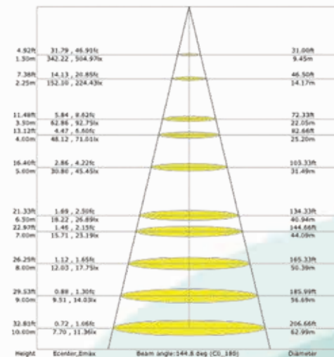
LX-Distance Diagram
