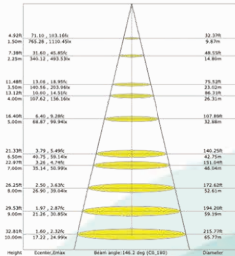
LX-Distance Diagram
