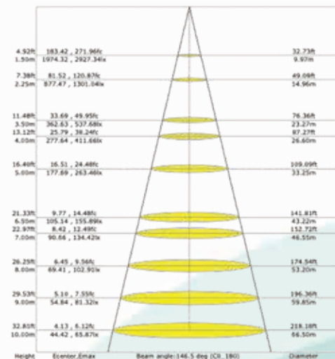
LX-Distance Diagram
