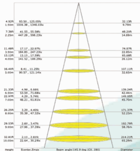
LX-Distance Diagram
